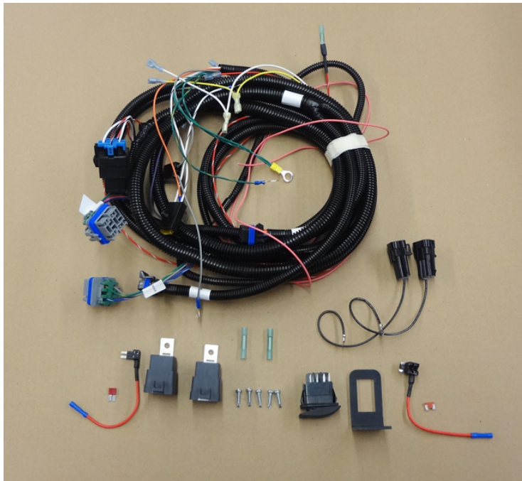
53807-M Kit
