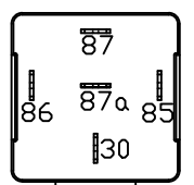
Low Beam Curb Side Relay
