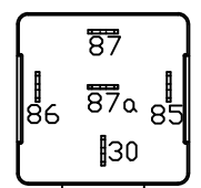
High Beam Curb Side Relay
