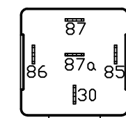
Low Beam Drivers Side Relay
