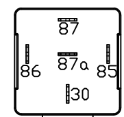
High Beam Drivers Side Relay
