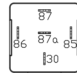
Low Beam Curb Side Relay
