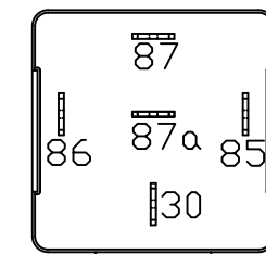
Low Beam Drivers Side Relay
