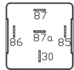
High Beam Drivers Side Relay
